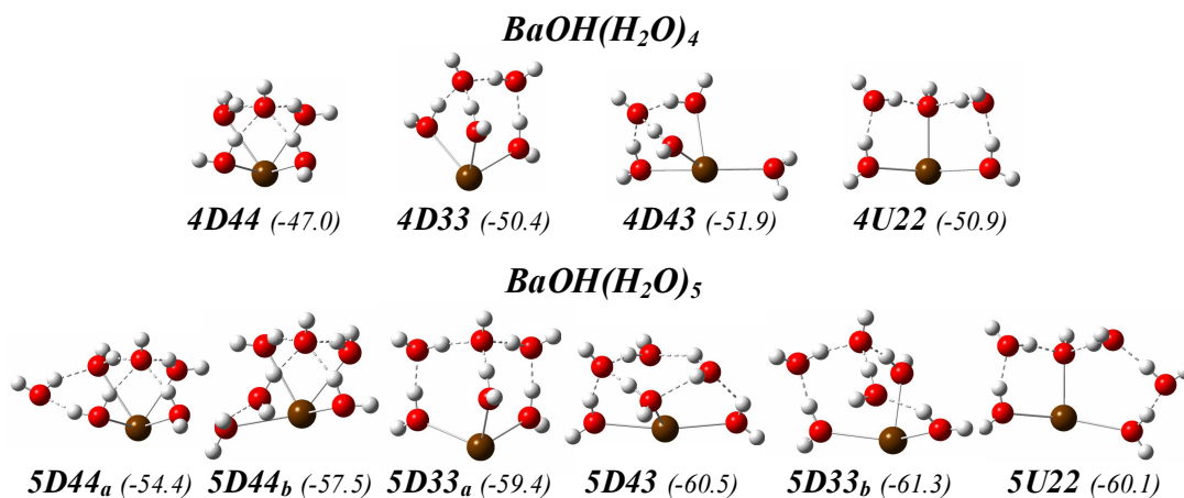
Figure 4. Same as Fig. 2, but for selected most stable BaOH(H_2O)_m ( m = 4 and 5 ) clusters. The binding energy (in \text{kcal mol}^{-1} ) next to the label of each structure was calculated at mPW1PW91 level. The results show an increase in the number of dissociated stable geometries as a function of m .
